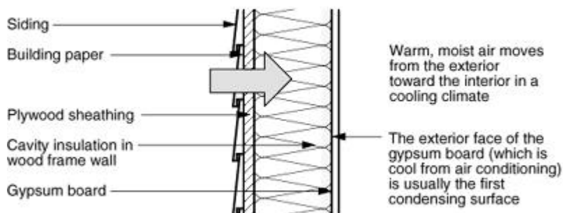
Figure 3: The exterior face of the gypsum board is usually the first condensing surface in a cooling-climate wall assembly.
